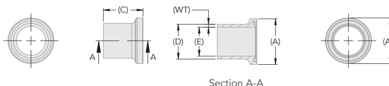
Type B – 50.5mm to 338.0mm Flange
