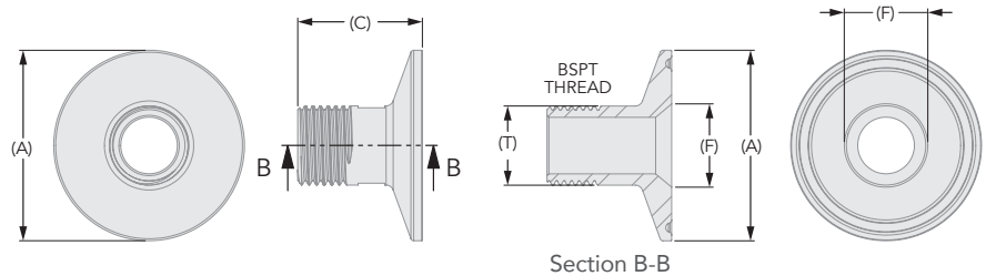
Type B – 50.5mm to 64.0mm Flange
