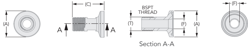
Type B – 50.5mm to 64.0mm Flange
